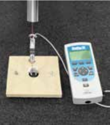
Device for high-heel test Fixing elements strength testing
