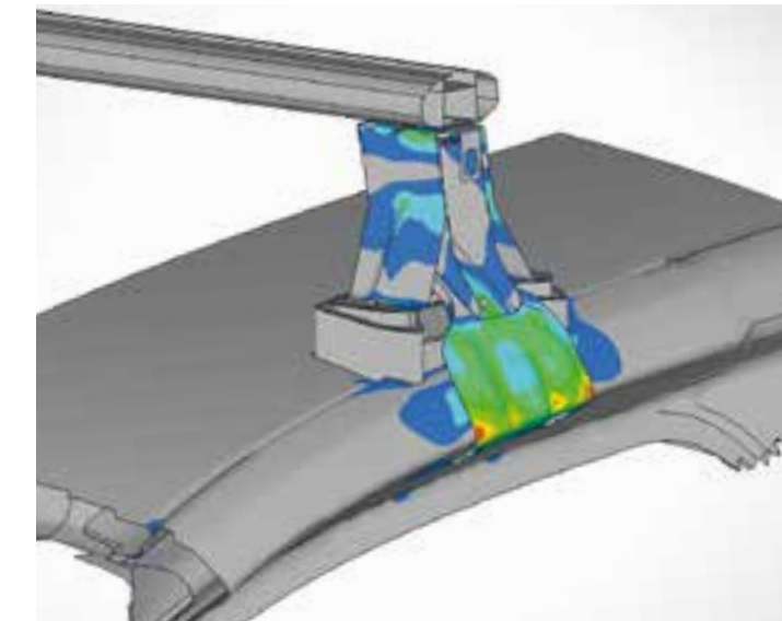
Map simulation of tension induced by tightening the roof rack
